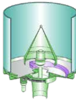
SILO DISCHARGE MACHINE
